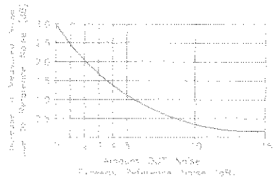
4 Increase in Measured Noise as Reference Source Noise Approaches OUT noise
