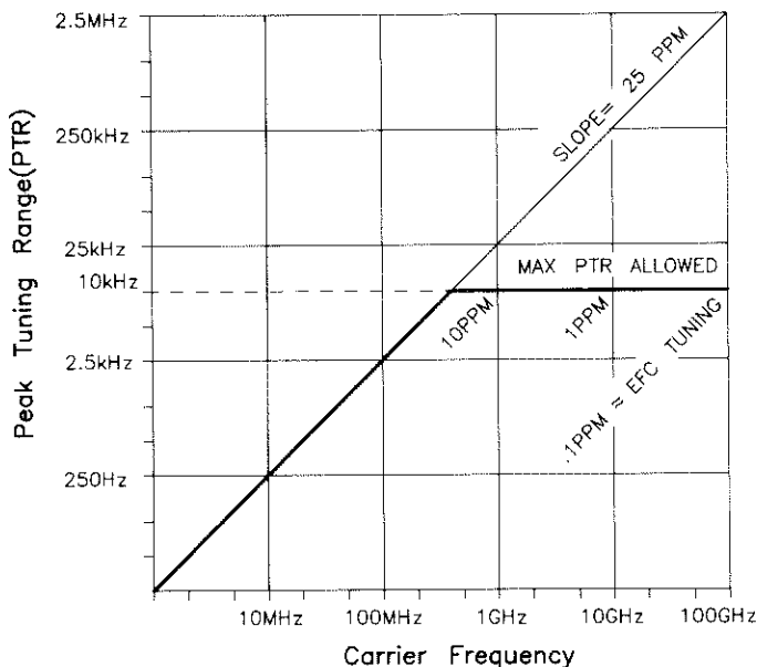
Figure 6-19. Graph of Limits for Maximum Peak Tuning Range Using EFC
