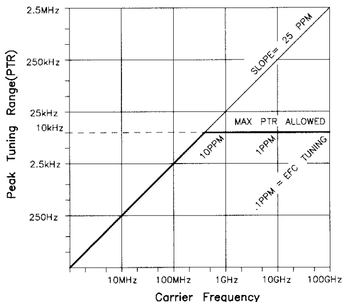
Figure 6-6. Graph of Maximum External Reference Tuning
